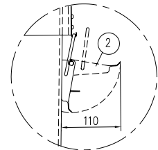
DETAIL CLOSING DEVICE M 1:5
